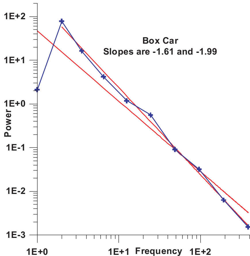
Figure 7. Power spectra from Table 3, using the random walk signal shown in Figure 6. Powers for various harmonic ranges are averaged and are plotted at the average harmonic value within each range. The left-hand point is for the fundamental (harmonic 1), the second point is for harmonic 2, the third point is for harmonics 3 to 4, the fourth point is for harmonics 5 to 8 etc. The red lines are best fitting lines through all points, and all but the fundamental, which has low power because a best fitting line was removed from the signal before taking the spectrum.
